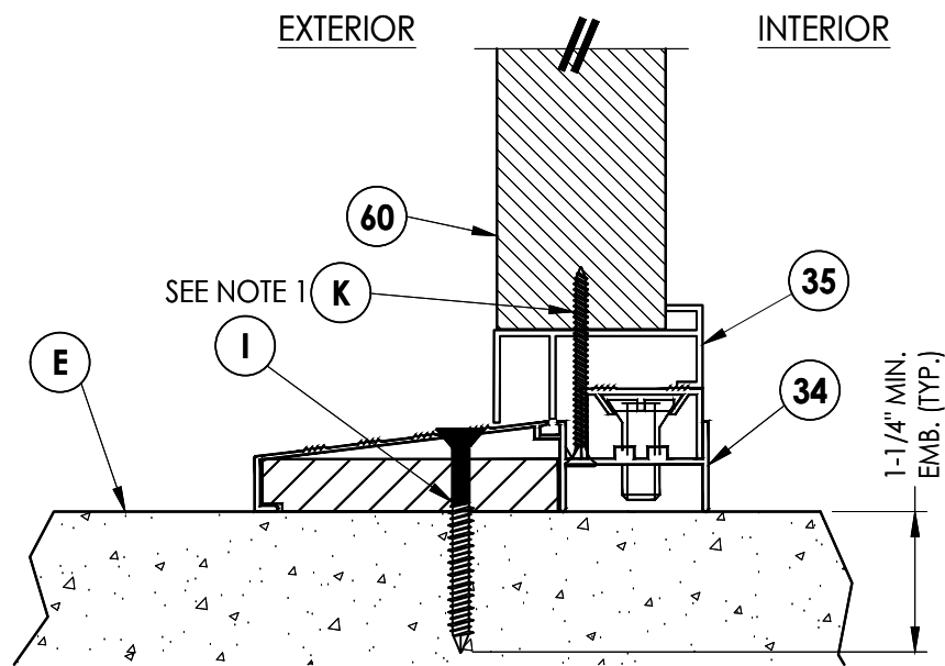
3 8 VERTICAL CROSS SECTION Inswing configuration
