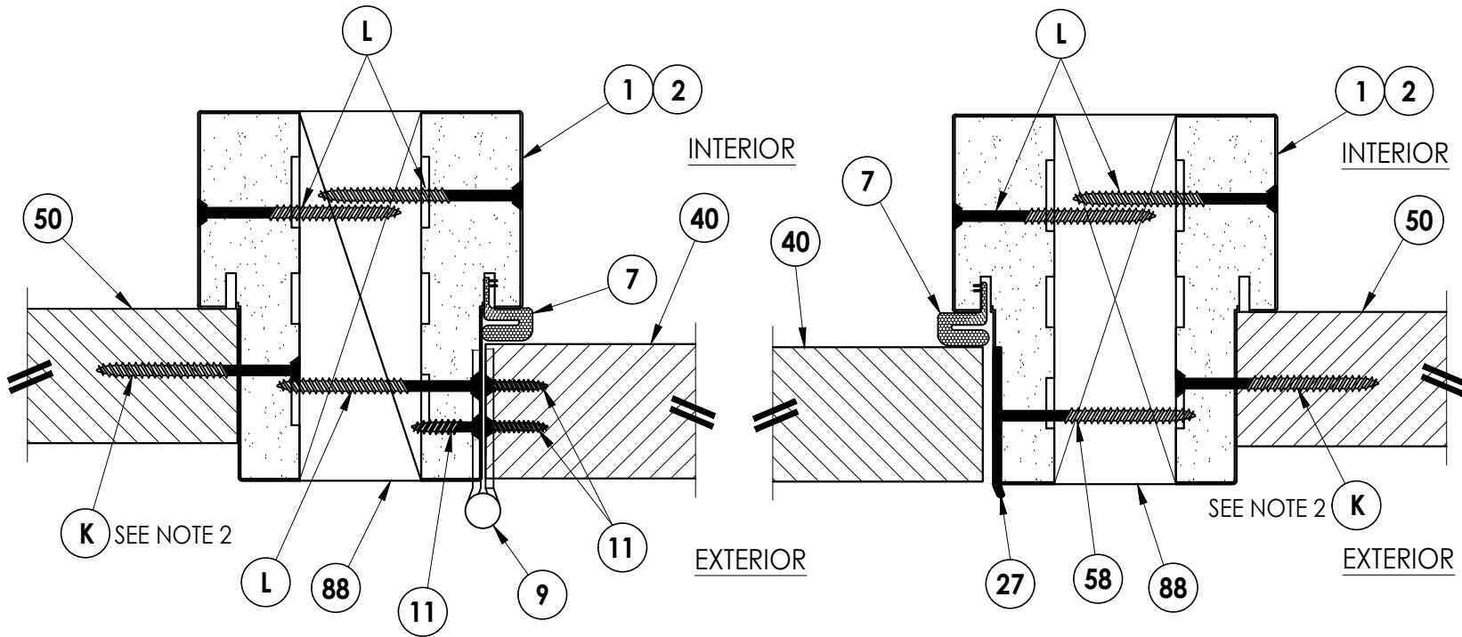
4 5 HORIZONTAL CROSS SECTION Outswing shown (Inswing similar)
