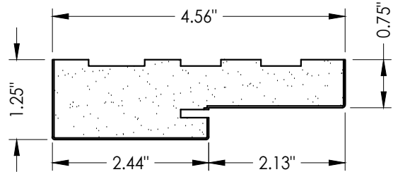
2 HEAD & SIDE Poly fiber jamb
