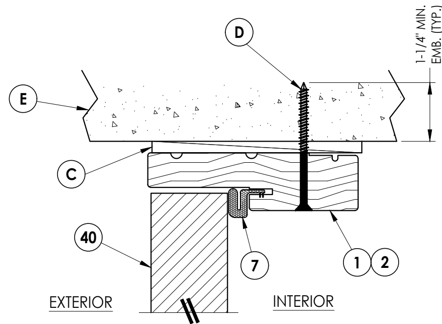
2 VERTICAL CROSS SECTION 7 Shown Direct to Masonry Outswing shown (Inswing similar)
